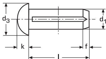
Grooved pins, round head
