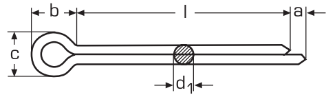
Split cotter pins
